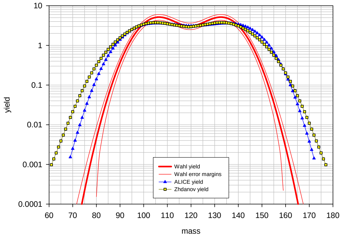
Benchmark B: ^{241}\text{Am} at 50 MeV, pre-neutron emission mass distribution
